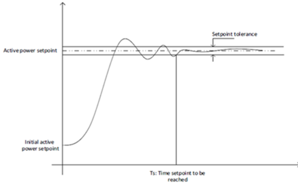
Figure 3: Tolerance and time duration for application of a new active power set point
