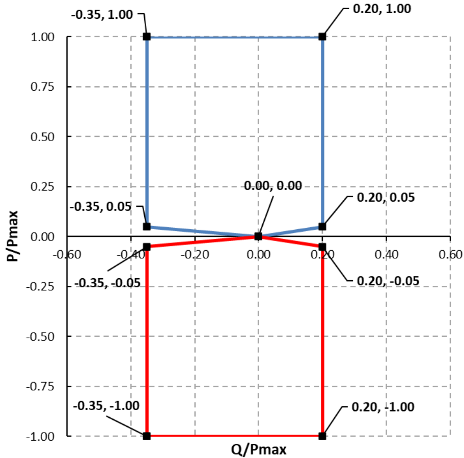
Figure 3: P-Q/Pmax-profile of ESMs connected at 150/400kV
