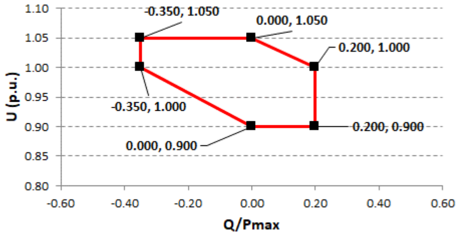
Figure 2: U-Q/Pmax-profile of ESMs connected at 400kV
