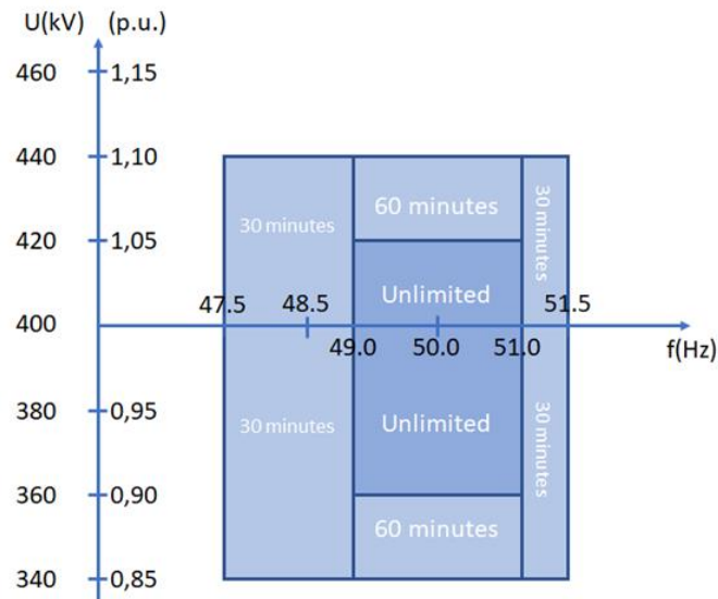
Figure 2: Minimum requirements for steady-state operation of PGMs connected at 400 kV, where U is the voltage at the CP (in kV) and f is the system frequency (in Hz)
